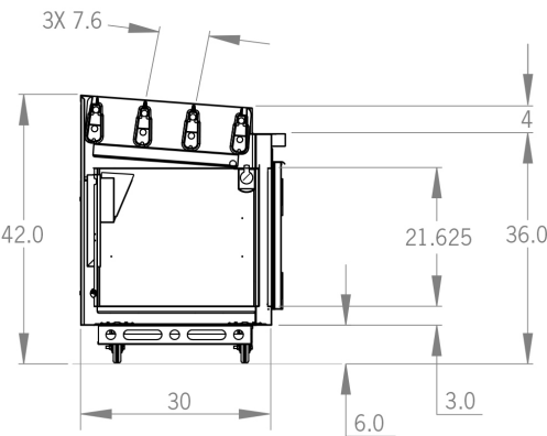
Section View
