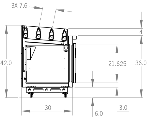
Section View
