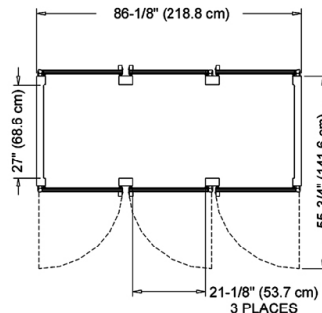
Plan - R/AHT132WP/UT
